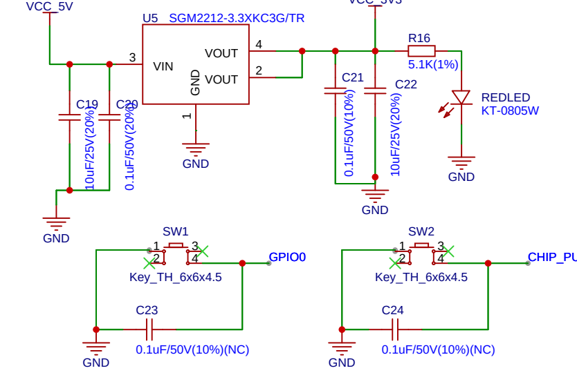
LDO, Boot & RST of ESP32-S3
