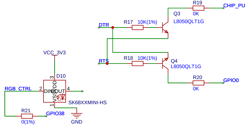
Auto Download Circuit & RGB LED of ESP32-S3
