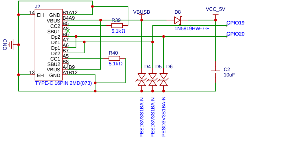
USB-UART & USB Port of ESP32-S3
