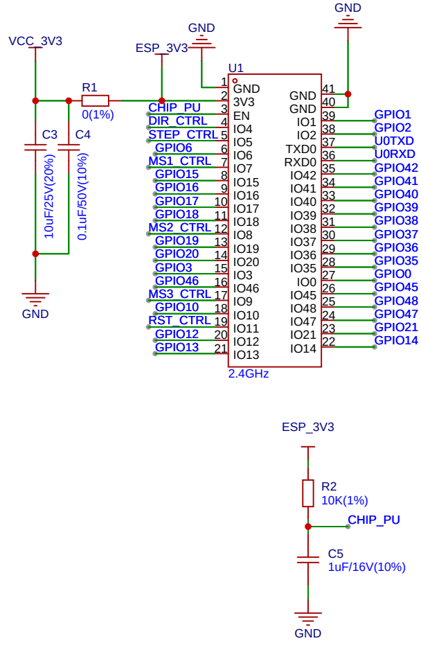
ESP32-S3-WROOM-1/1U Module
